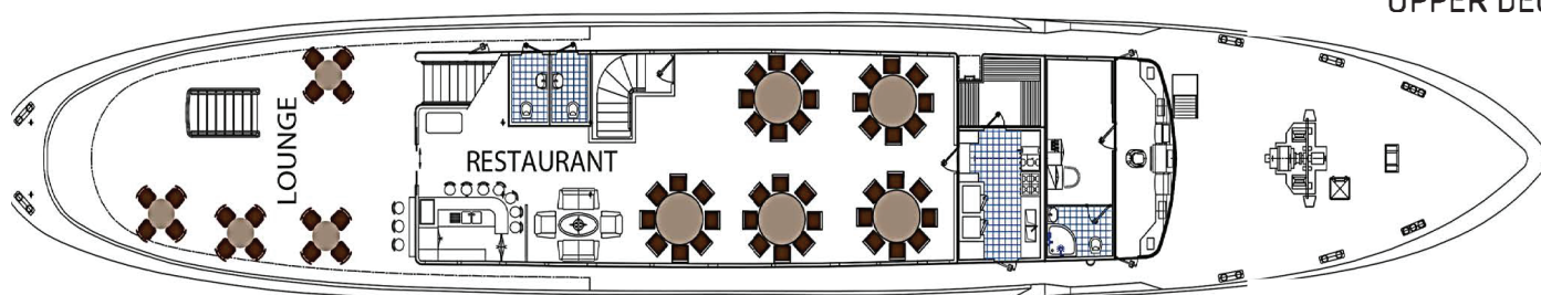
UPPER DECK
